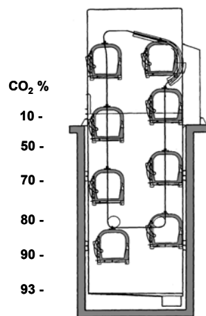
Figure 9-4. Principles in the carbon dioxide gradient in a paternoster carbon dioxide stunning system
